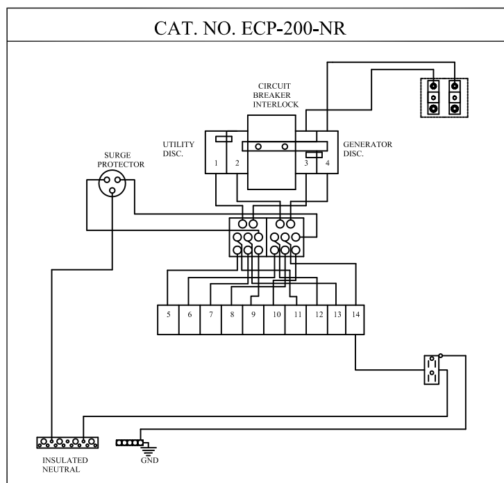
TYPICAL WIRING DIAGRAM
